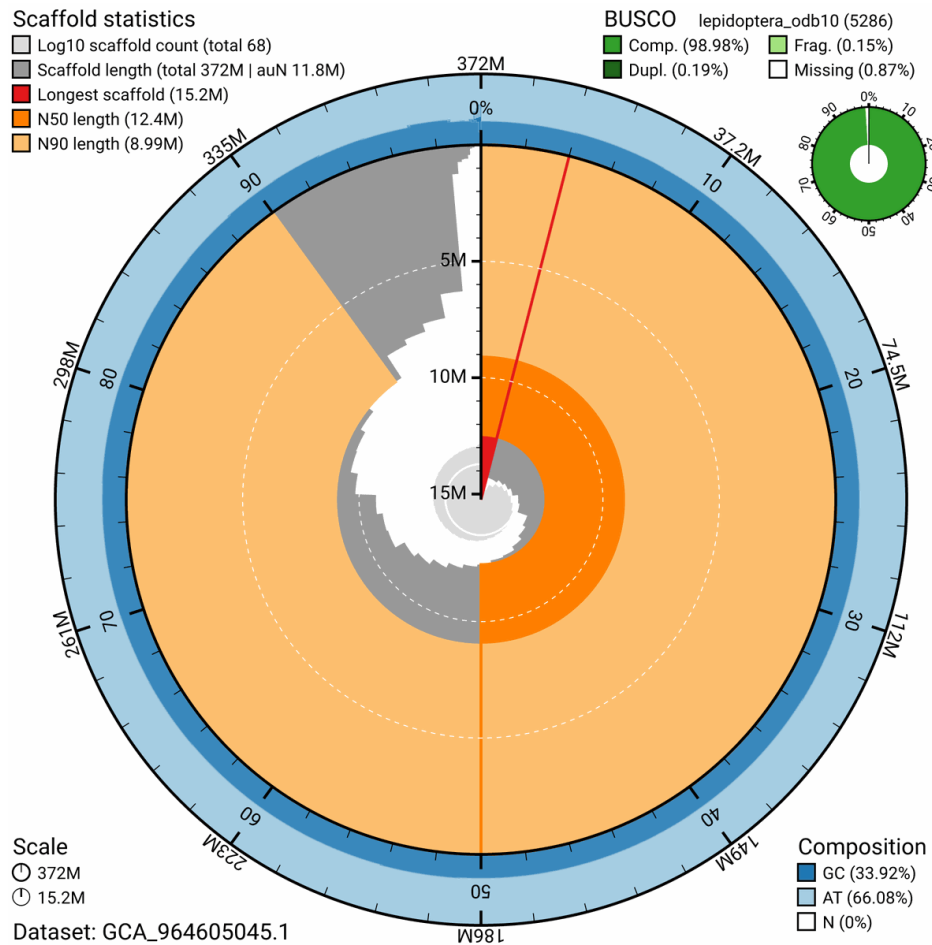
Figure 6. Assembly metrics for ilEucInsu1.hap1.1, the haplotype 1 assembly. The BlobToolKit snail plot provides an overview of assembly metrics and BUSCO gene completeness. The circumference represents the length of the haplotype 1 assembly, and the main plot is divided into 1,000 bins around the circumference. The outermost blue tracks display the distribution of GC, AT, and N percentages across the bins. Scaffolds are arranged clockwise from longest to shortest and are depicted in dark grey. Scaffold length is shown on a linear radial scale, scaled to the longest scaffold. Red shading indicates the longest scaffold, and the deeper orange and pale orange shading represent the N50 and N90 lengths. The summary statistics include scaffold auN, the area under the scaffold Nx curve. The light grey spiral at the centre shows the cumulative scaffold count on a logarithmic scale. A summary of complete, fragmented, duplicated, and missing BUSCO genes in the lepidoptera_odb10 set is presented at the top right. The assembly can be explored interactively in the BlobToolKit viewer .
