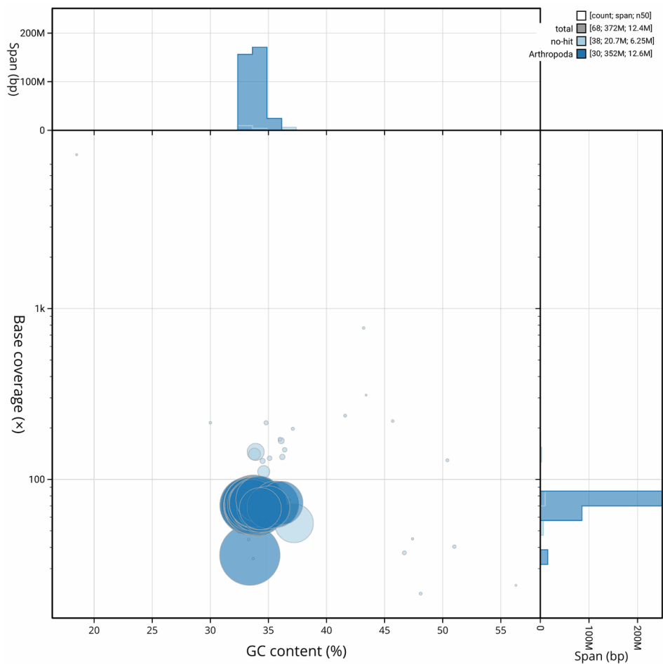
Figure 7. BlobToolKit blob plot for ilEucInsu1.hap1.1 , the haplotype 1 assembly. The plot shows base coverage (vertical axis) and GC content (horizontal axis). Circles represent scaffolds; marker area is proportional to scaffold length, and colour indicates taxonomic assignment. The histograms along the axes display the total length of sequences distributed across different levels of coverage and GC content. The assembly can be explored interactively in the BlobToolKit viewer .
