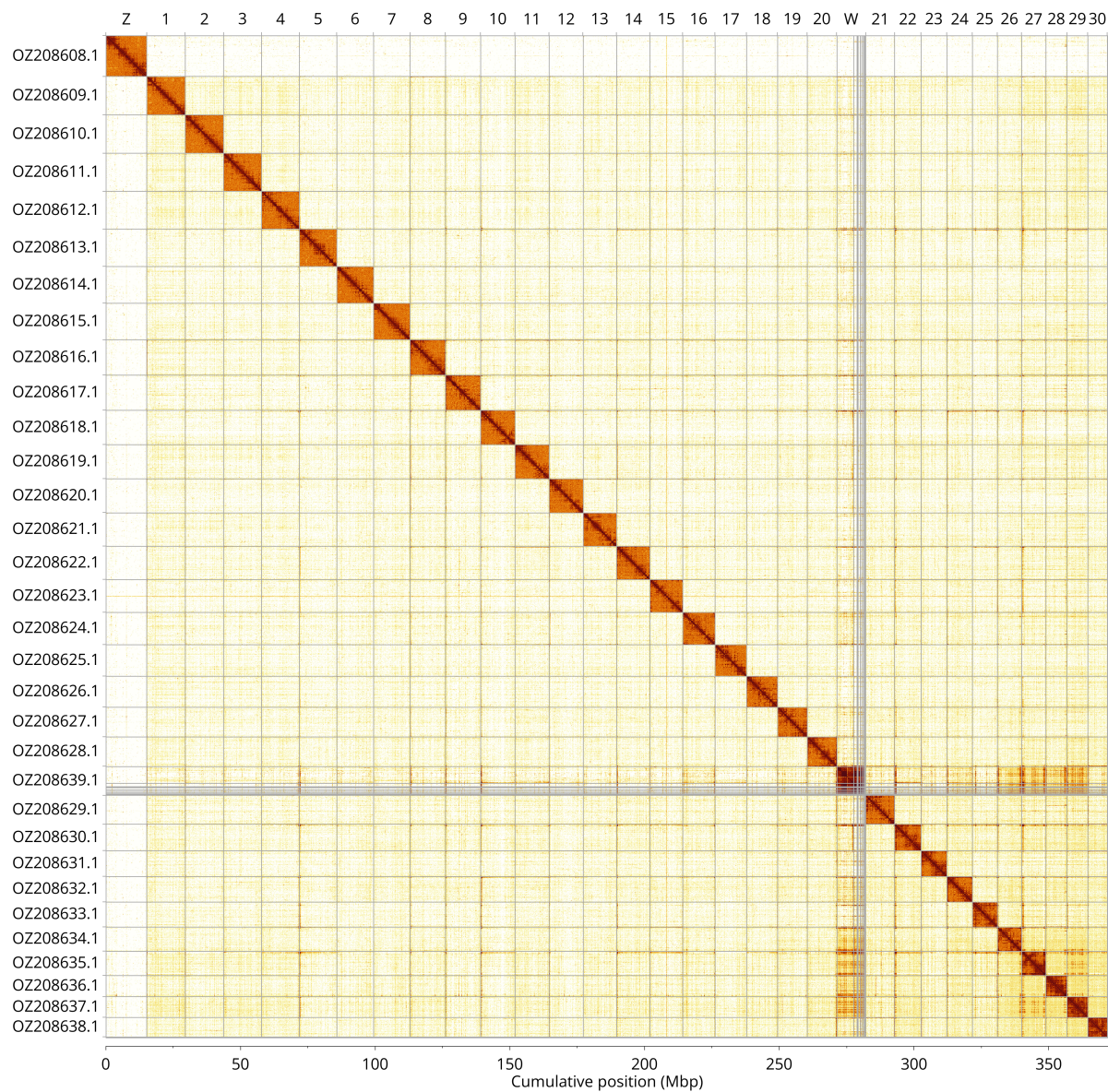
Figure 3. Hi-C contact map of the E. insularis haplotype 1 assembly. Assembled chromosomes are shown in order of size and labelled along the axes. The plot was generated using PretextSnapshot.
