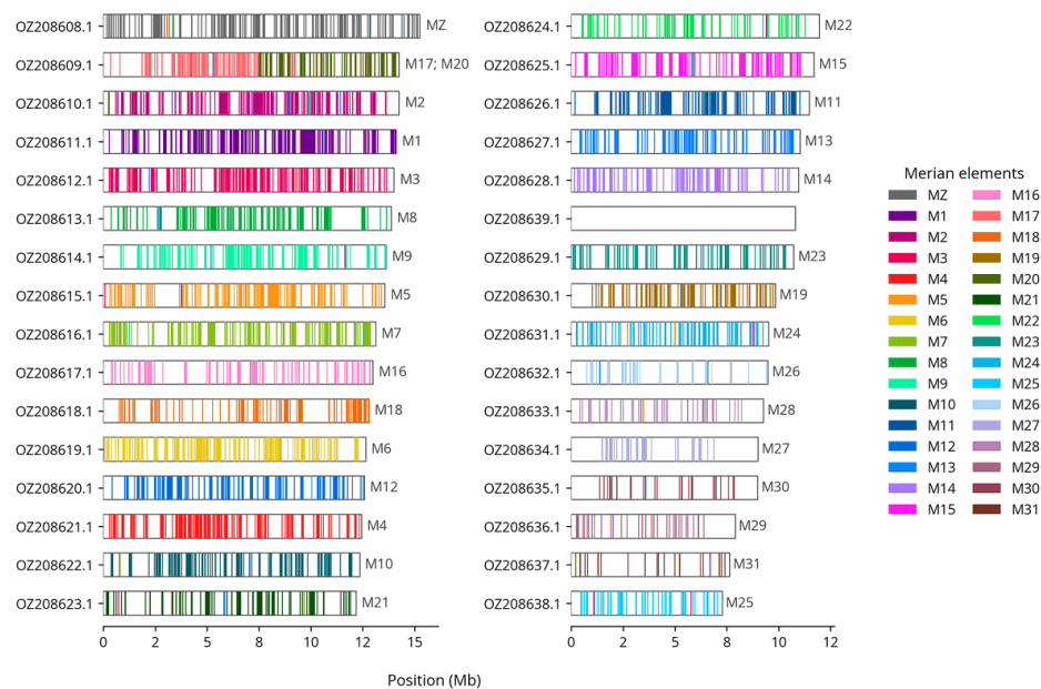
Figure 4. Merian elements painted across chromosomes in the ilEucInsu1.hap1.1 haplotype 1 assembly of E. insularis . Chromosomes are drawn to scale, with the positions of orthologues shown as coloured bars. Each orthologue is coloured by the Merian element that it belongs to. All orthologues which could be assigned to Merian elements are shown.
